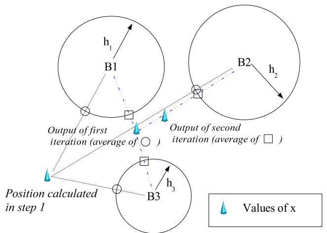
Fig. 2. Two iterations of the PB algorithm in 2 dimensions. The node projects itself on a hypersphere of radius h_u around every beacon B_u . The input to the next iteration is the average of these projections. This implements a gradient-descent minimization of h(\cdot) defined in (1).
